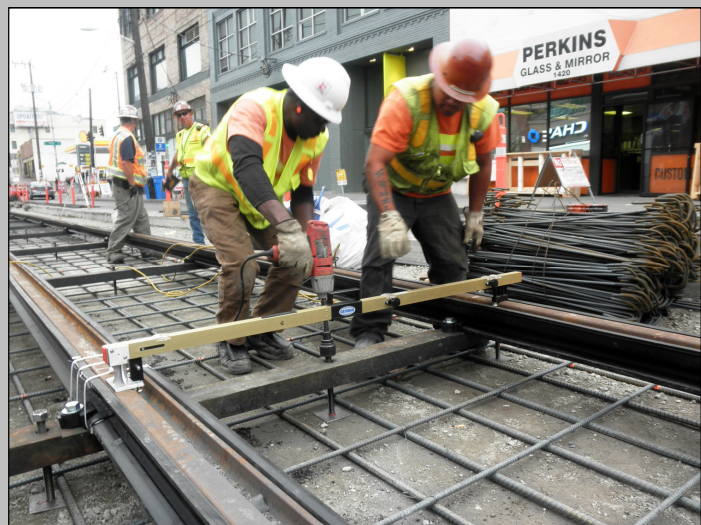
Adjusting rail to final grade
