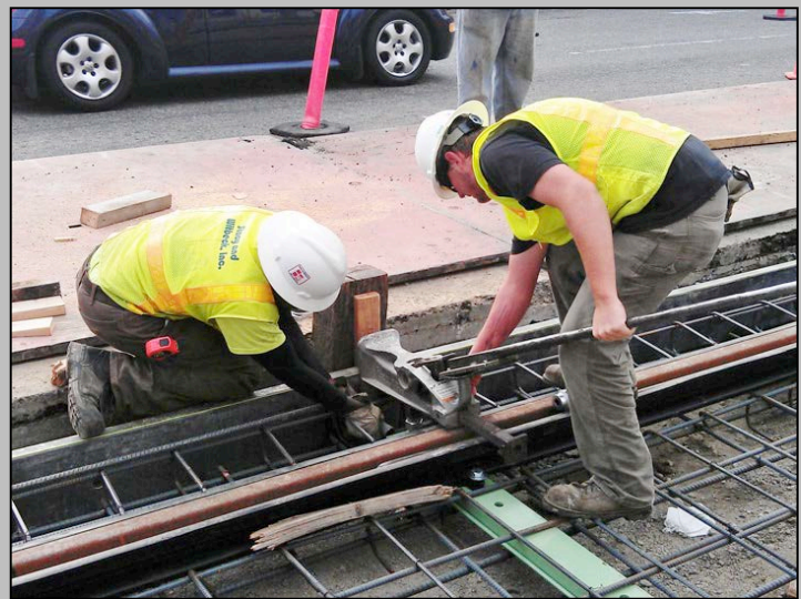
Using a track jack to align the rail
